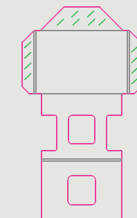
Base EB 4/0 - 0,51x0,91m - rodapé
