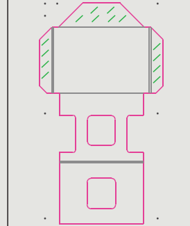
Base Papelão EB 4/0 - 77x94cm x6700 - rodapé
